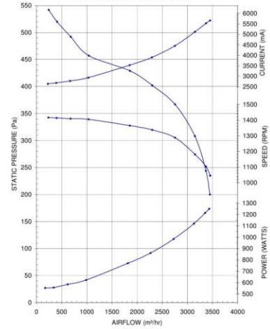
TORIN SIFAN AFZUIGMOTOR 4250 M3/H DDC270-270-550W-4P-1SP 230V 50Hz 16MFD 5,6A
