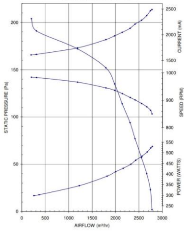
TORIN SIFAN AFZUIGMOTOR 2500 M3/H DDC241-241-245W-6P-1SP 230V 50Hz 8MFD 2,4A
