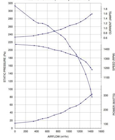
TORIN SIFAN AFZUIGMOTOR 1500 M3/H DDN201-178 230V 50Hz Motor: SPC1412 (147w 4p 1s 5uf HE)
