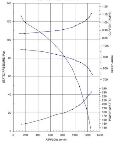
TORIN SIFAN AFZUIGMOTOR 1200 M3/H DDN200-178-73W-6P-1SP 230V 50Hz 3MFD 1.1A
