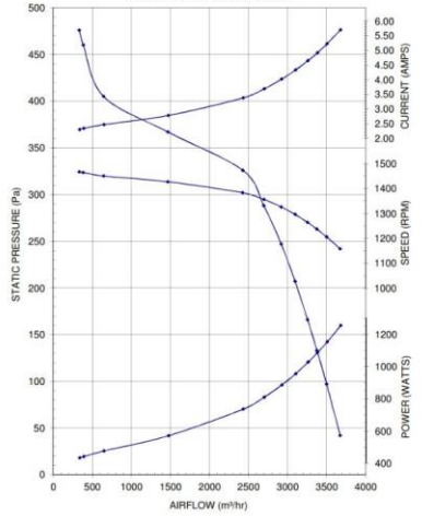
TORIN SIFAN AFZUIGMOTOR 3250 M3/H DDC241-241-550W-4P-1SP 230V 50Hz 16MFD 6.0A
