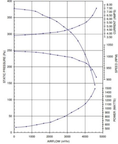
TORIN SIFAN AFZUIGMOTOR 5000 M3/H DDC321-241-750W-6P-1SP 230V 50Hz 16MFD 7.5A
