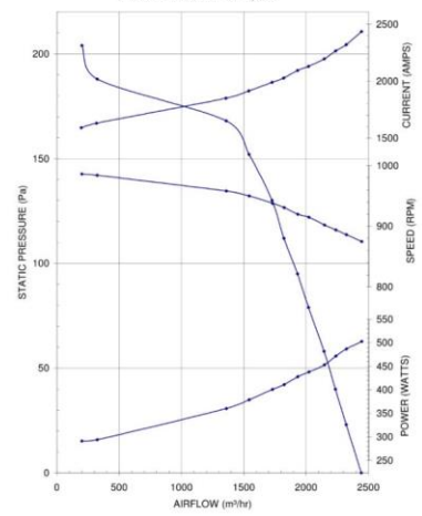
TORIN SIFAN AFZUIGMOTOR 2000 M3/H DDC241-181-245W-6P-1SP 230V 50Hz 8MFD 1,5A
